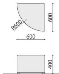
RO-NR600
