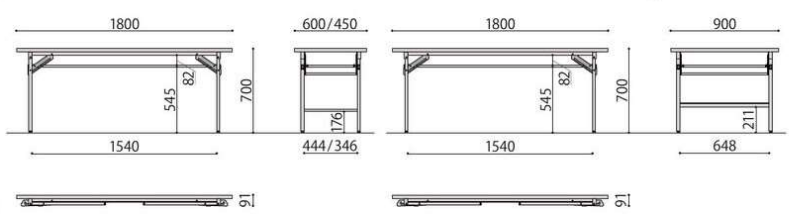
VKT-1860S-1845S
